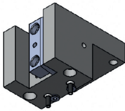
M06-S011250E TURNING TOOL HOLDER HOLE SECTION 25X25MM TSUGAMI# 3295-H260
