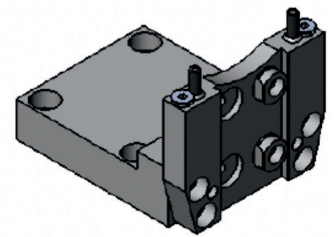
M06-S030320E CUT-OFF TOOL HOLDER HOLDER SECTION 32MM TSUGAMI# 3295-H250
