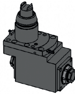
M06-R211320E RADIAL OFFSET DOUBLE 90 DEGREE TOOL HOLDER Tool Clamp ER32A/ER32A
