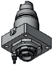
M06-A110320E AXIAL 0 DEGREE TOOL HOLDER Tool Clamp ER32A TSUGAMI# 3295-Y161
