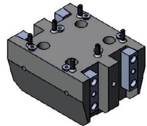
M06-S014250E TURNING TOOL HOLDER_QUAD HOLE SECTION 25X25MM
