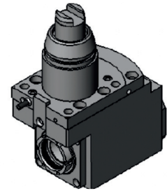
M06-R111320E RADIAL OFFSET 90 DEGREE TOOL HOLDER Tool Clamp ER32A
